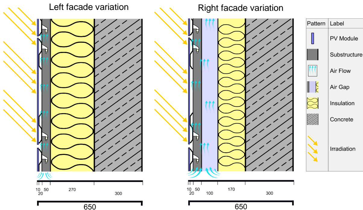
Figure 4: Schematic facade cross section of both variations of the module substructure
