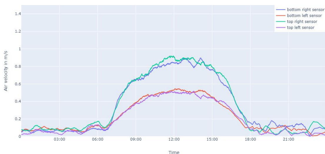
Figure 27: Average air velocity of the rear-ventilation on the 1 st of March
