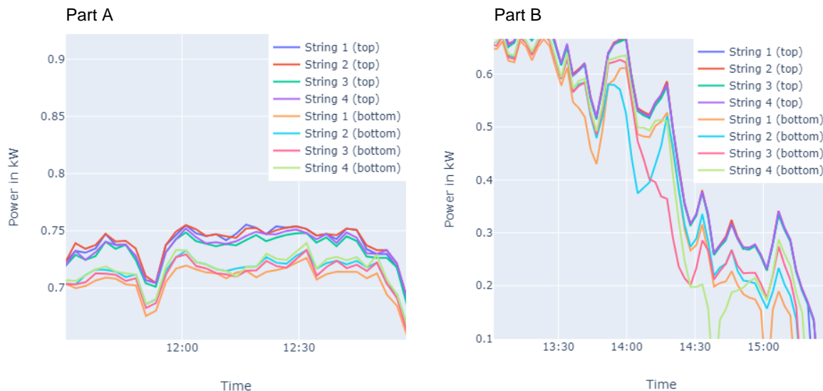
Figure 14: PV power in the area under investigation for each string on the 13 th of February
