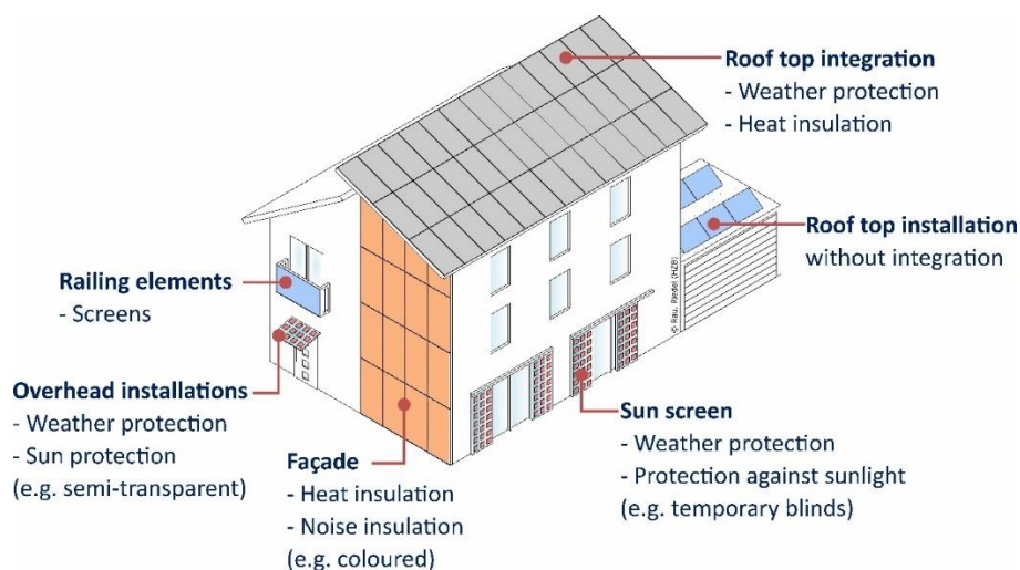
Figure 1: Schematic illustration of the different opportunities to integrate photovoltaics into the building © HZB
