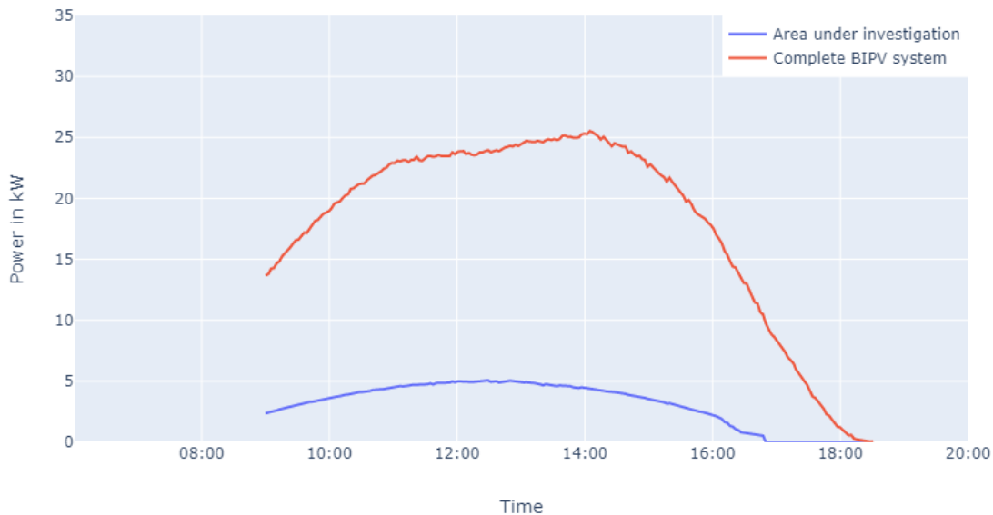
Figure 11: Comparison of data from the AC and DC measurement devices on the 24 th of March
