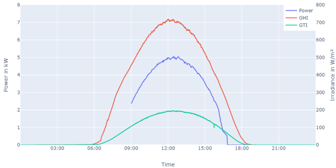
Figure 12: Total PV power in the area under investigation in contrast to the irradiance on the 24 th of March
