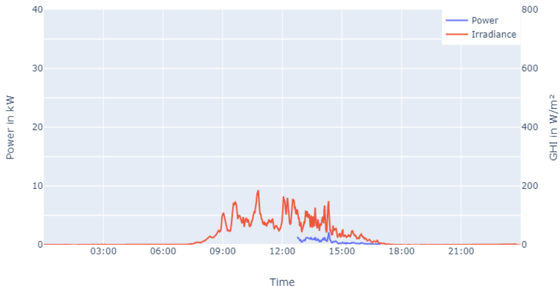
Figure 13: Total PV power in the area under investigation in contrast to the irradiance on the 16 th of February
