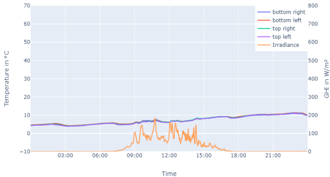
Figure 18: Average string temperature and global tilted irradiance on the 16 th of February
