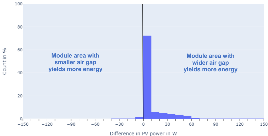
Figure 32: Difference in PV power from two different facade substructure variations (02.01. – 02.04.2022)
