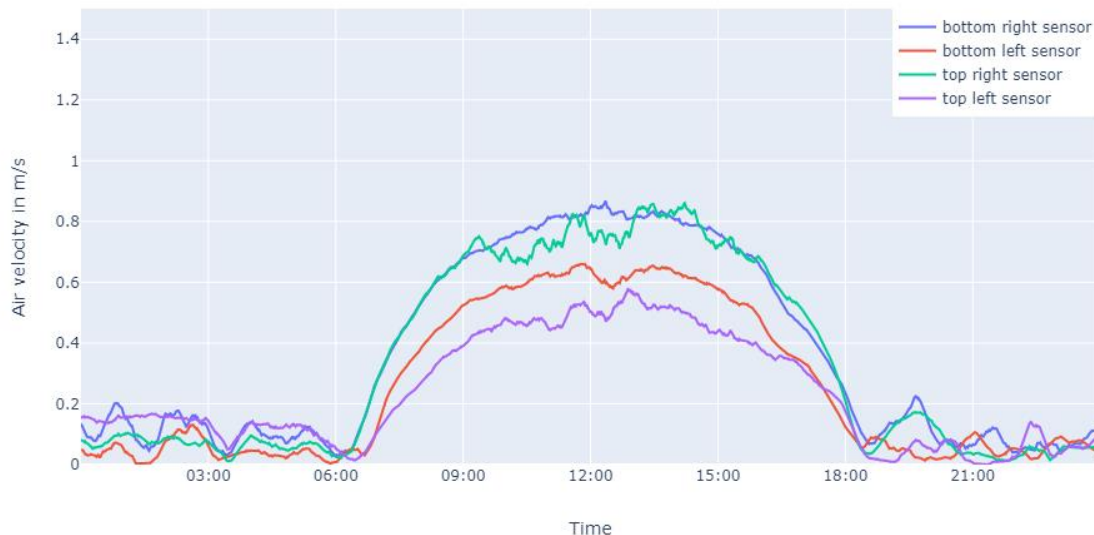
Figure 20: Average air velocity of the rear-ventilation on the 24 th of March
