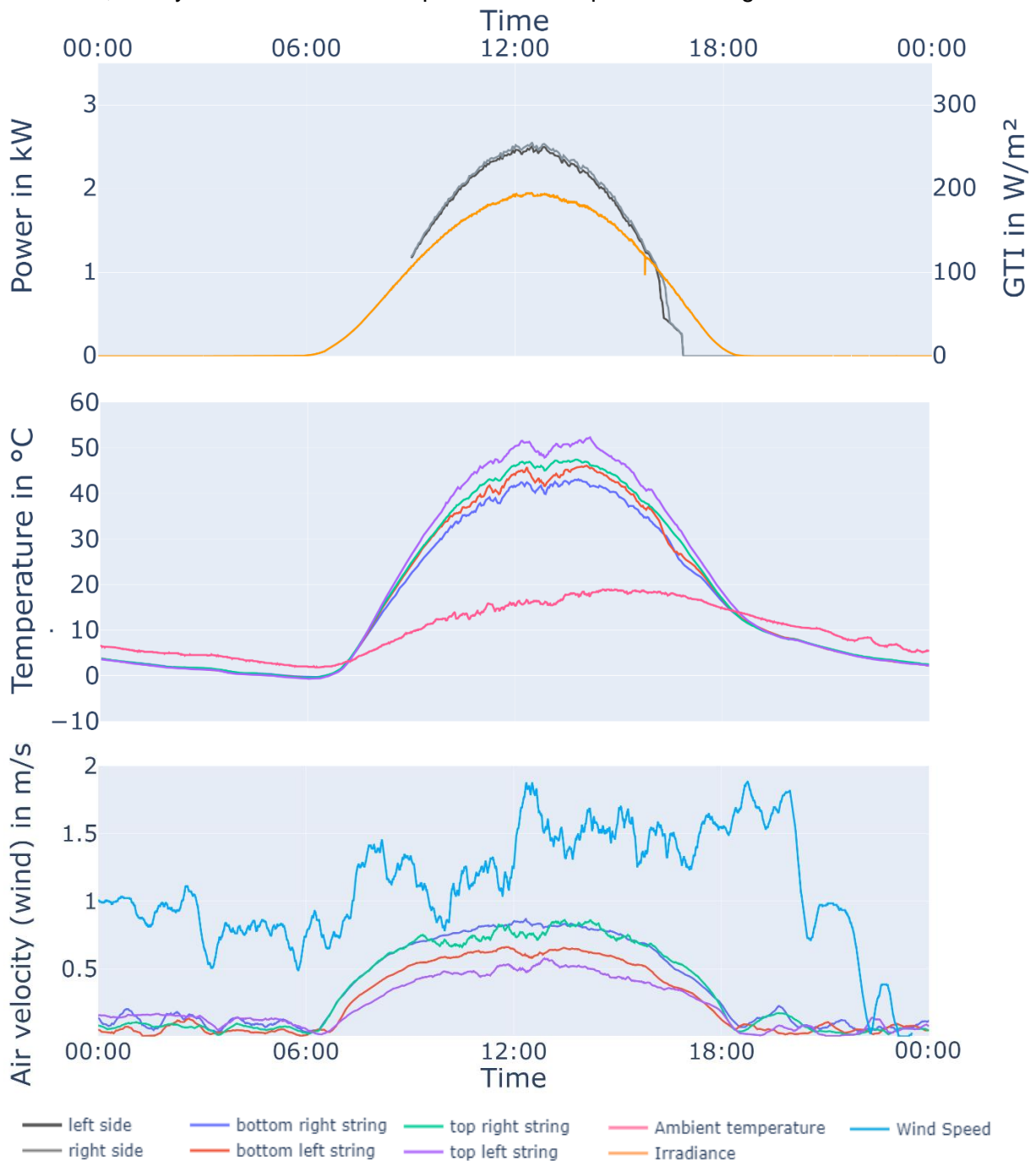
Figure 26: Overview over every measurement on the 24 th of March
