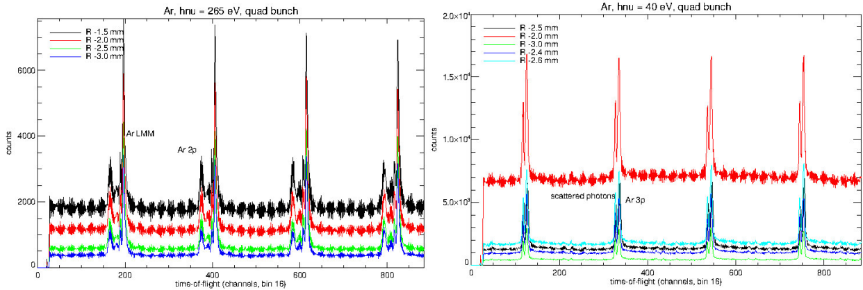
Figure 2: Electron time-of-flight spectra of Ar photo and Auger lines from island orbit (quad bunch) and main orbit for different settings of the right-hand side ID blade (R). Separation can be improved at the expense of few bunch signal, but is not perfect. Quality of the separation (peak height vs. flat background) is dependent on photon energy (left h\nu=265 eV, right h\nu=40 eV).
