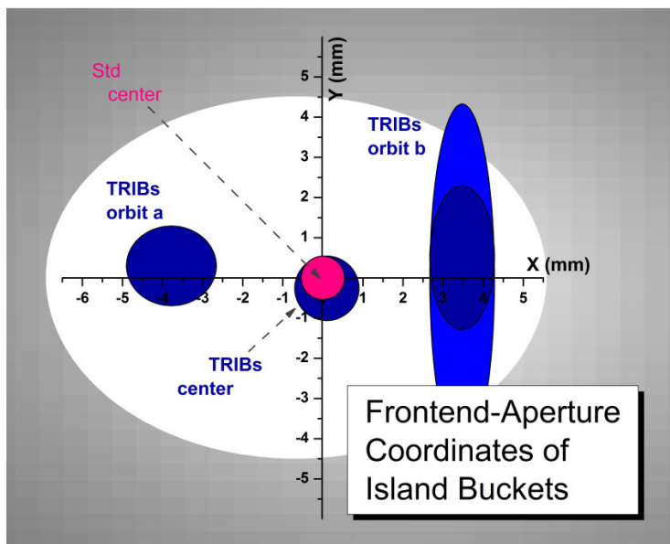
Figure 1: Size (FWHM) and positions of different beam spots determined from front-end aperture (ID blade) settings and photo-current measurements. The origin of co-ordinates is given by the standard beam center in decay mode. The central TRIBS orbit is slightly larger and two of the TRIBS island buckets (orbits a plus b) have clearly been detected. Orbit (a) has been used for the subsequent TOF experiments and for orbit (b) only the x-distribution has been determined.
