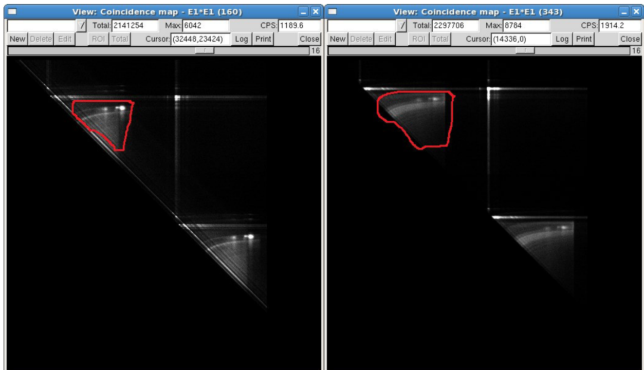
Figure 3: Electron coincidence spectra in a short time-of-flight vs. long time-of-flight representation encompassing two BESSY periods (1600 ns). True autoionization signal from molecular oxygen (bright spots marked by red boundaries) can be seen in the spectrum acquired in twin-orbit mode (left) similar to earlier measurements in single bunch (June 2016, UE56/2). (Contrast in the rhs panel is worse because of a background from water clusters.)
