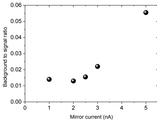
Figure 2. Ratio of background to the signal maximum indicating a good signal to background ratio below 2 nA.
