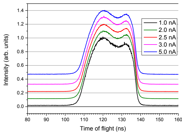
Figure 1. Time of flight spectra for different slit settings indicated by the increasing mirror current. The spectrum remains similar while the constant time-independent background from the multibunch train increases.
