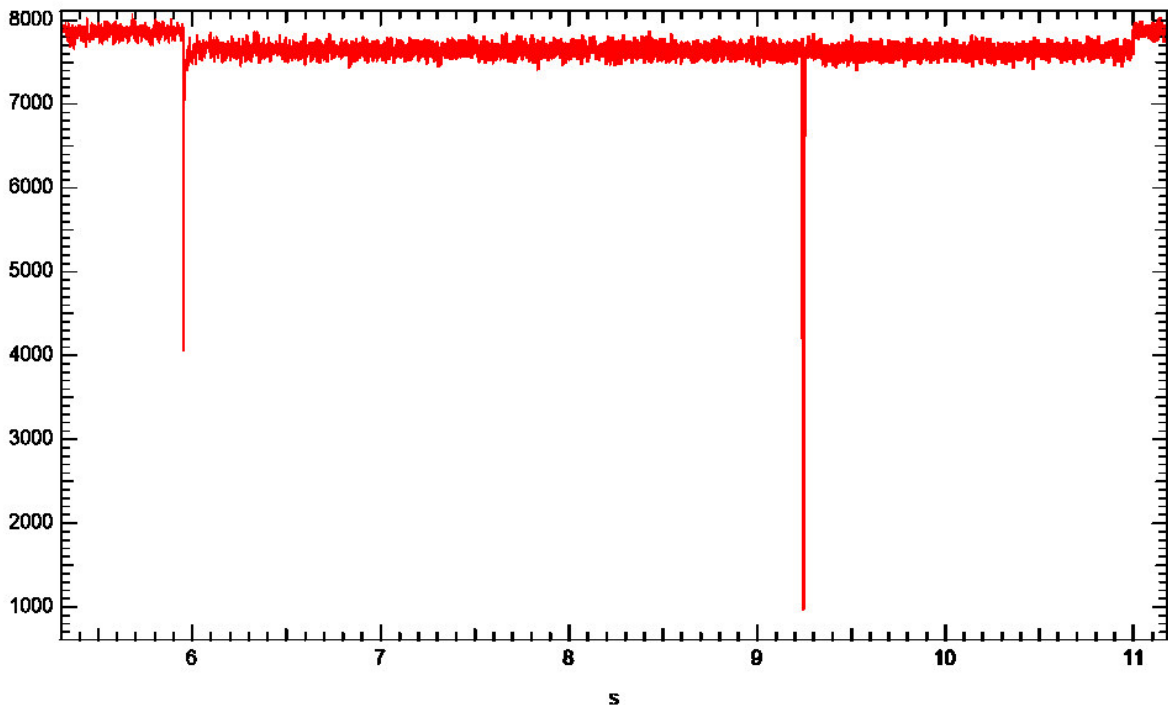
Fig. 1: Image intensity as measured at MAXYMUS during an injection. Visible are 2 dips (top-up and island merge) as well as a drop in intensity while the island was merged into the main orbit
