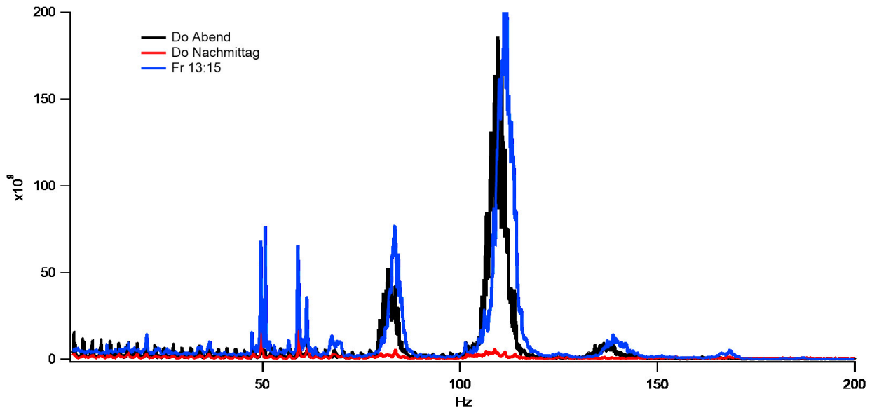
Fig. 3: Noise spectrum (arbitrary units with fast orbit feedback off (red line) and on (blue/black)). Noise level was not suitable for spectromicroscopy (very bad image distortion) with fast orbit feedback on, but otherwise fine.
