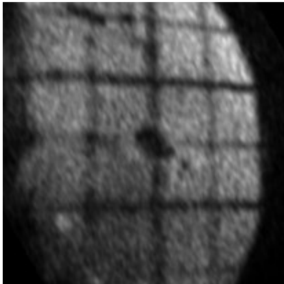
Figure 3. Image of the Chessy sample with the grid introduced into the backfocal plane. Photoelectrons excited with 18 eV. Image averaged over 100 meV close to the photoemission threshold ( E_B = 13 eV). Data accumulated for 10 minutes. The sharp image of the grid proves the possibility to perform momentum microscopy.
