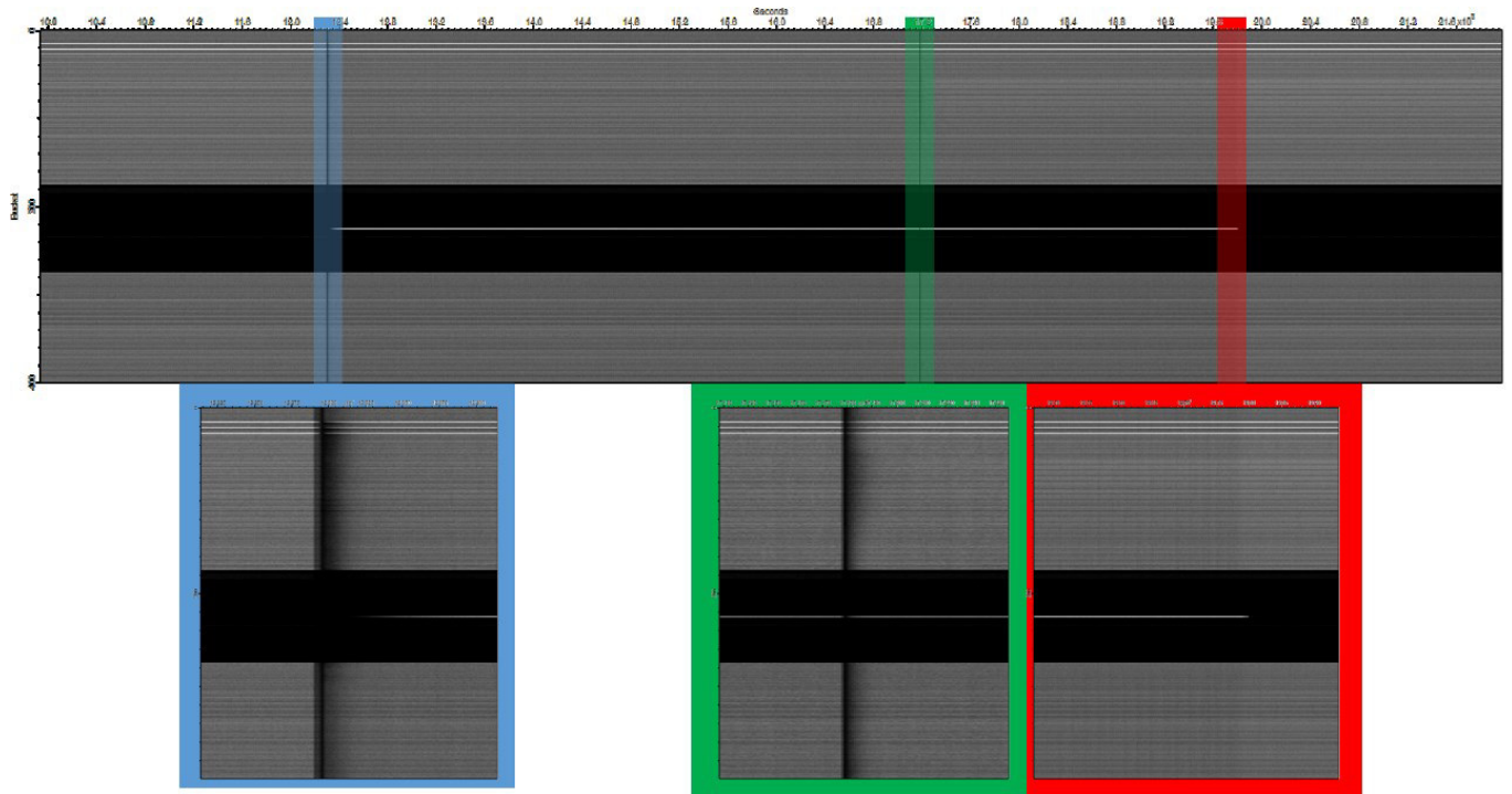
Fig. 2: Injection analyzed at bunch level. Vertical axis synchrotron bunch, horizontal time (1ms/pixel). Blank of the Multibunch train can be seen about 25ms before arrival of the island into the main orbit (blue cut-out), with notable differences in length depending on the position in the multibunch train. Green cutout shows the injection, red the un-merge of the island at the end of the injection cycle. Noise can be seen in the red cut-out due to the beamline BPC being confused by the beam shape during the merger
