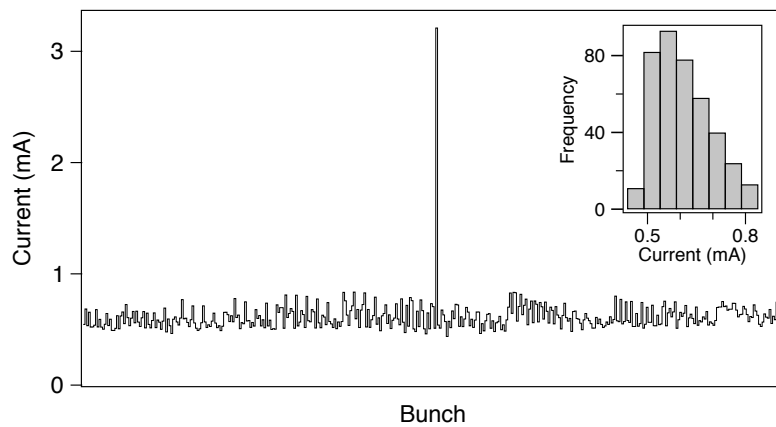
Figure 3: CUMZR:MBcurrent snapshot from (23/2/2018). Inset: Histogram of the bunch intensities excluding the single high intensity bunch.
