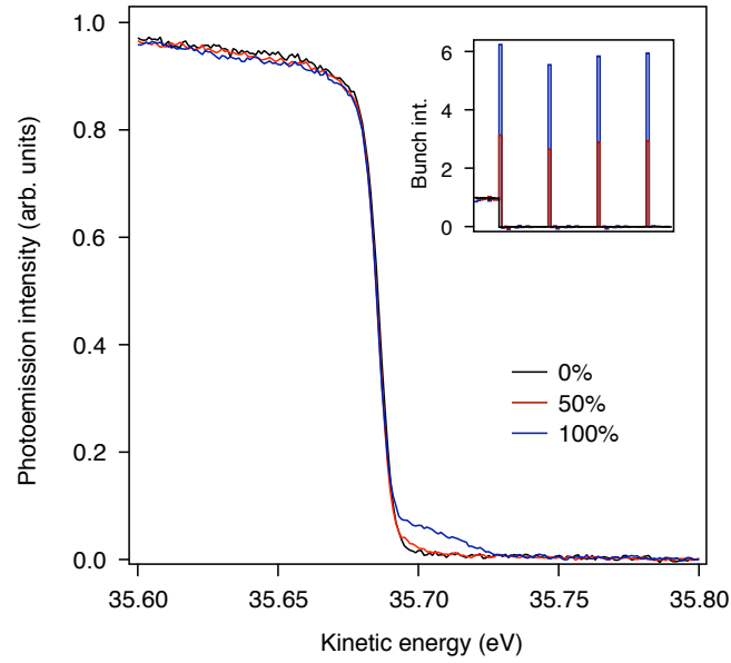
Figure 2: Effect of the hybrid bunch intensity on photoelectron spectra. Black curve is obtained with a storage ring filling of 300 equally intense bunches. Red and blue spectra taken with four additional bunches of approximately three and six times higher intensity (inset).
