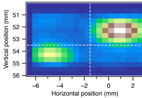
Figure 1: Intensity from UE-112 at 70 mm gap (22/2/2018 ~ 13:45; all current carried in island orbit) mapped with the 100 \mu\text{m} front-end pinhole. Dashed white lines indicate the coordinates of the beam center in normal operation.
